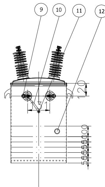
LV BUSHING TERMINAL DETAIL
